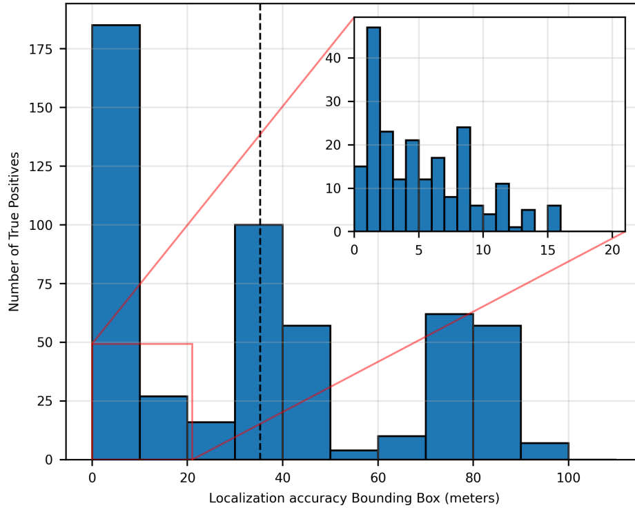
Figure 27: Localization accuracy (bounding box) across experiments. The main histogram shows the localization accuracy of a true positive (TP) detections calculated as the distance from the center of the bounding box of the controlled release source. The insert shows 1 meters resolution for distances between 0 meters to 20 meters.
