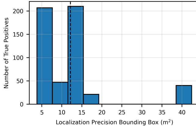
Figure 29: Localization precision (bounding box) across experiments
