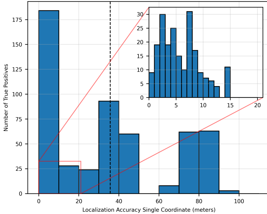
Figure 26: Localization accuracy (single coordinate) across experiments. The main histogram shows the localization accuracy of a true positive (TP) detections calculated as the distance from reported coordinates to the controlled release sources. The insert shows 1 meters resolution for distances between 0 meters to 20 meters.
