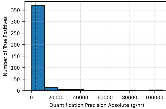
Figure 24: Quantification precision (absolute) across experiments
